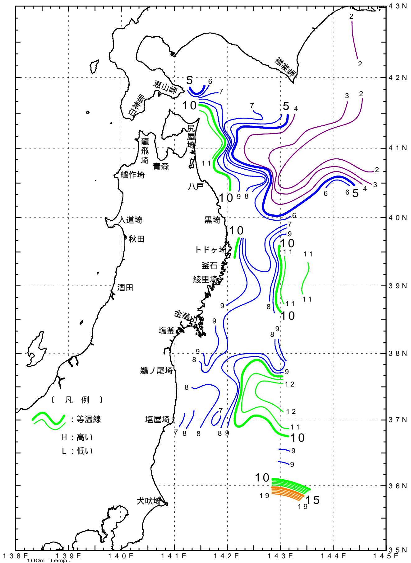
【100m層水温水平分布図( )】2008/6/13-6/26
