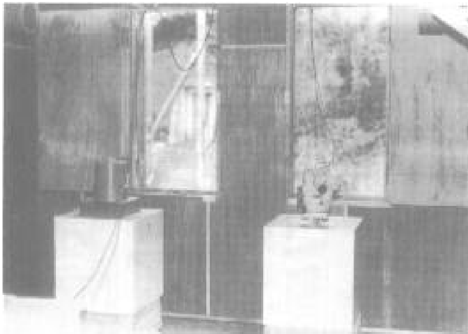
Magnetometer mounted on the Instrument Piers of the Absolute Observation House
