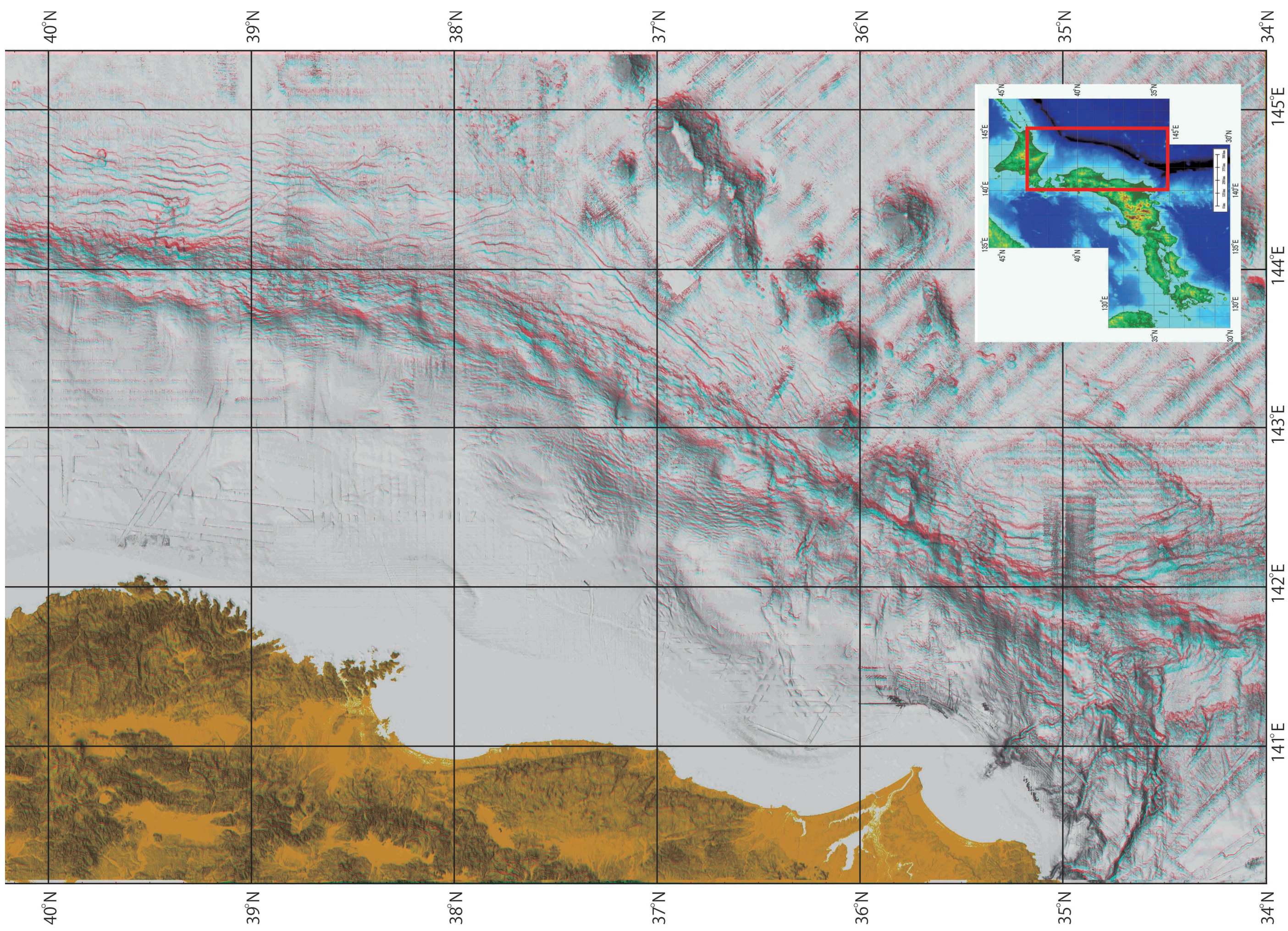
Fig. 7 Anaglyph image of the entire Japan Trench area
